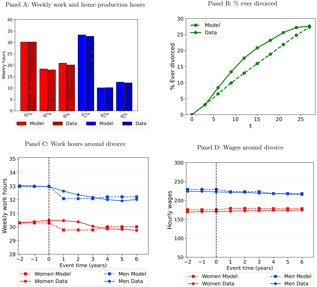
FIGURE 5: Model fit
